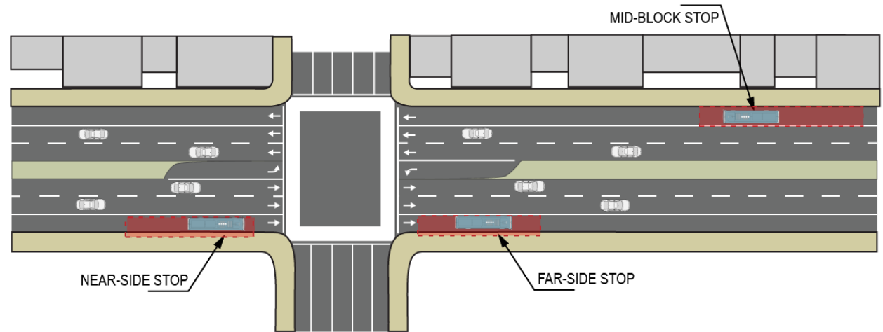
Figure 2.1 Far-side, Near-side and Mid-block Located Bus Stops 2
