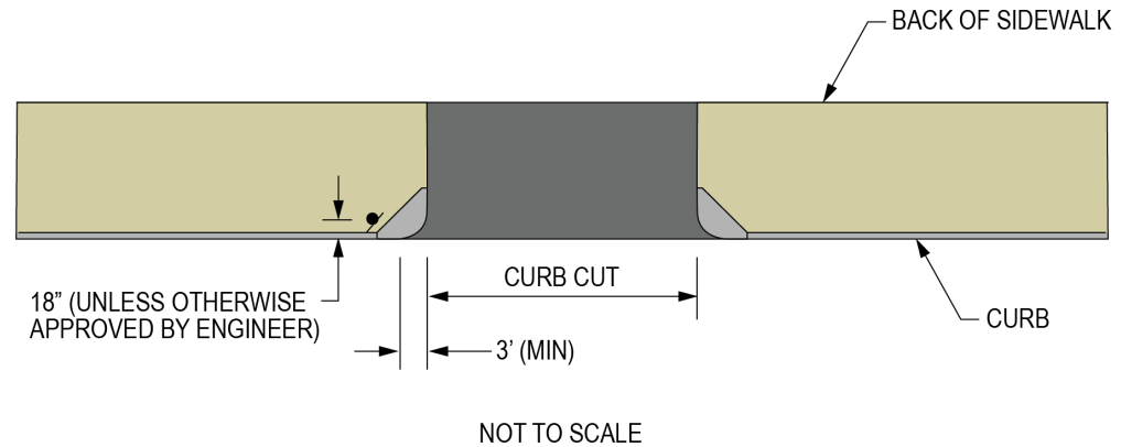
Figure 4.4 Bus Stop Sign Placement at Driveway
