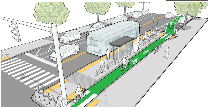
Figure 7.4 Floating Bus Stop
