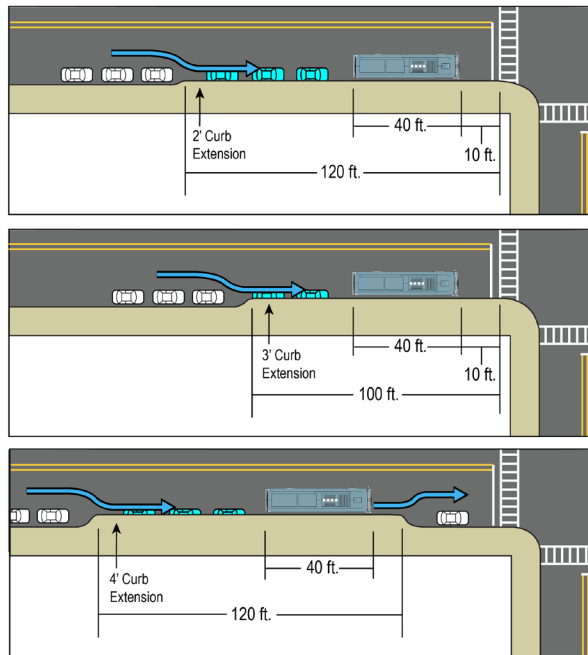
Figure 2.14 Partial Curb Extension Lengths and Parking Impacts 15
