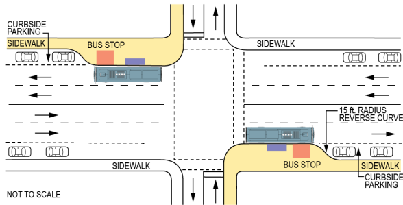
Figure 2.13 Bus Stop Curb Extension Far-side 14
