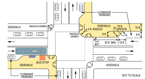
Figure 2.12 Bus Stop Curb Extension Near-side 13
