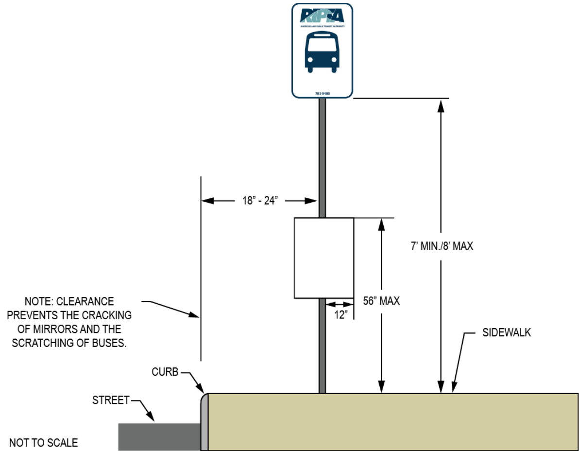
Figure 4.3 Bus Stop Sign and Post Placement 24
