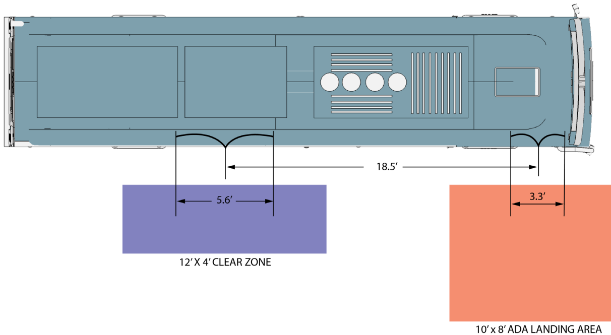
Figure 3.1 Landing Area and Clear Zone
