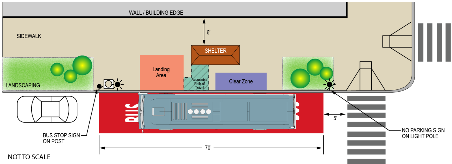
Figure 7.1 Ideal Bus Stop Layout
