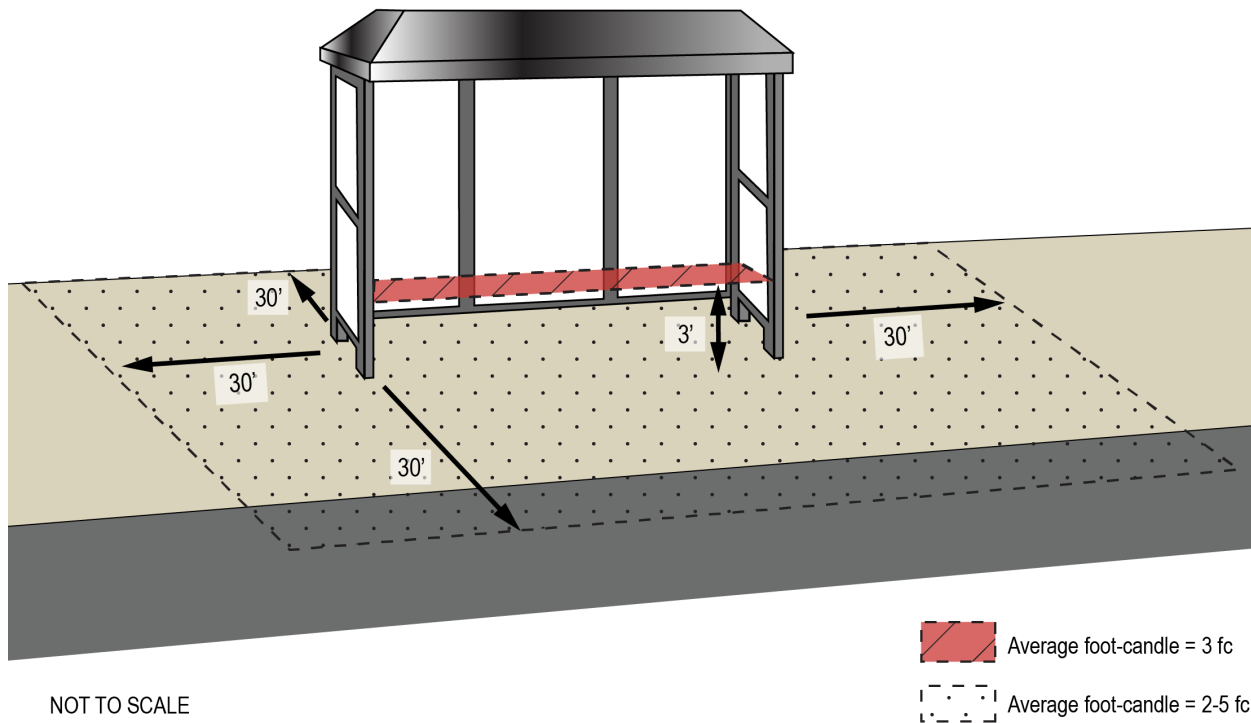
Figure 6.1 Shelter Lighting Guidelines
