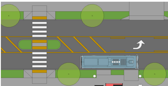
Figure 2.3 Bus Stop in Travel Lane
