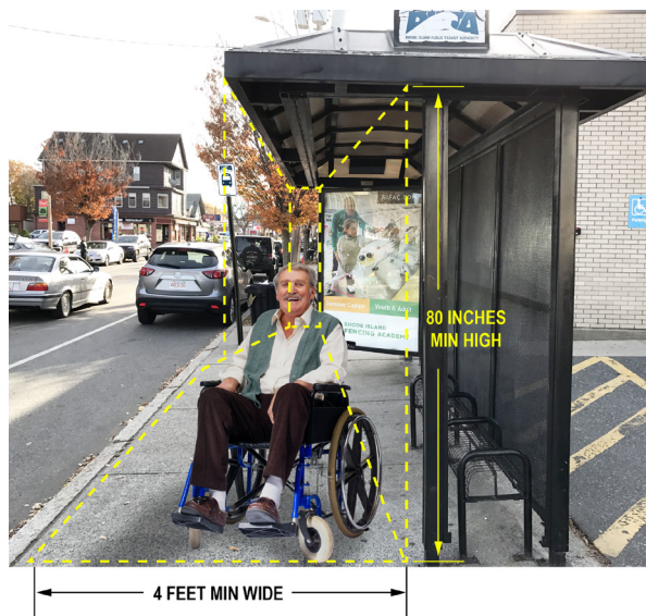
Figure 3.4 Pedestrian Vertical and Horizontal Clearances 22
