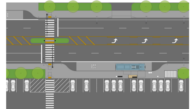
Figure 2.6 Bus Stop Pull Out
