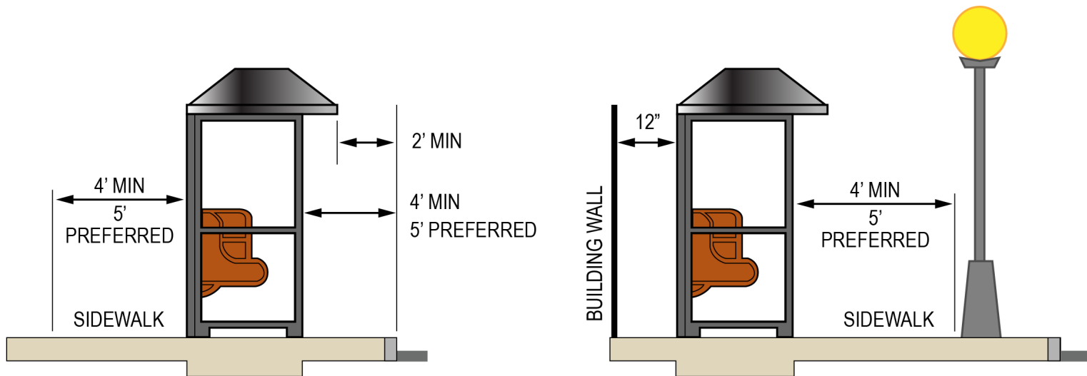
Figure 6.2 Key Shelter Clearances 28
