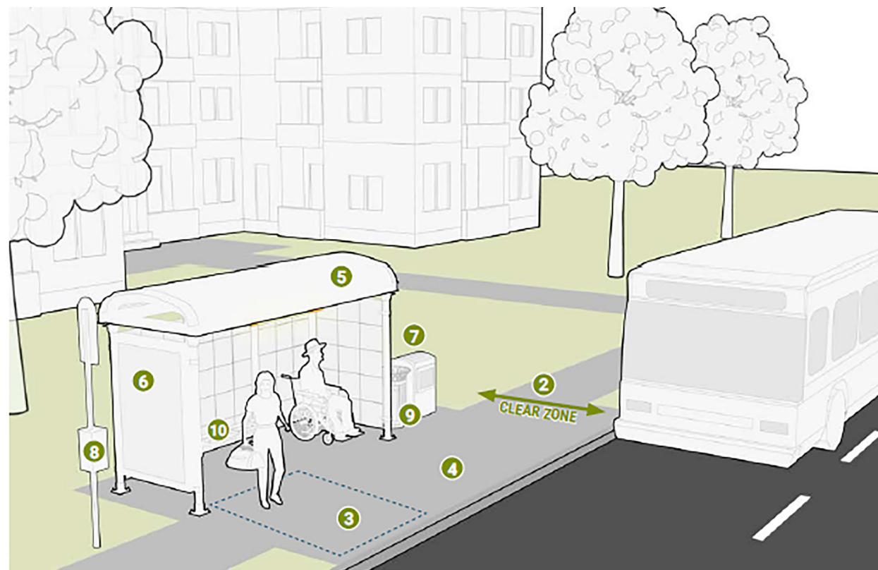
BUS STOP ON ROAD WITHOUT SHOULDER
