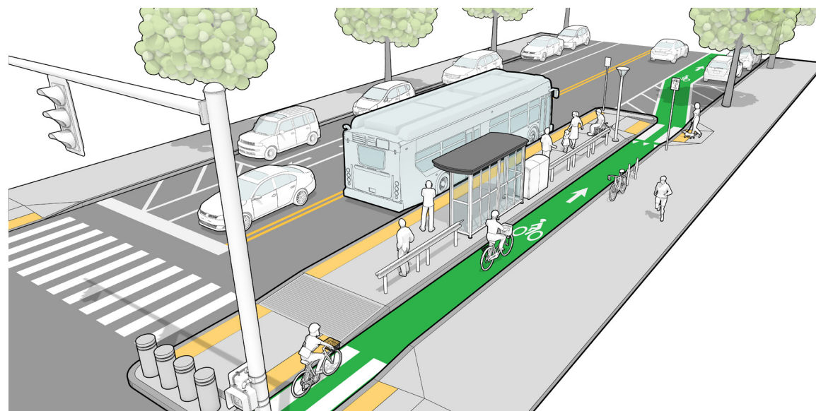
Figure 5.5 Floating Bus Stop
