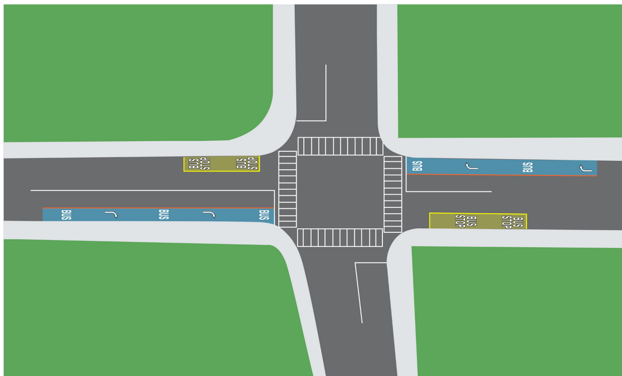
Figure 5.7 Bus Queue Jump Lane Shared with Right Turn Lane
