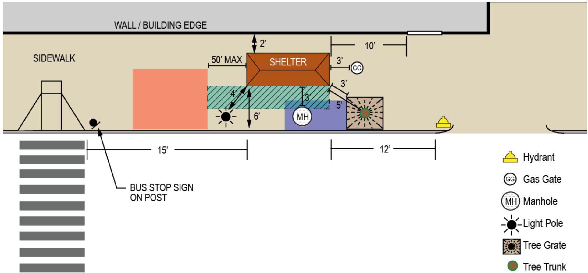
Figure 6.3 Detailed Shelter Clearances 30
