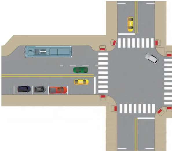
Figure 2.8 Far-side Partial Open Bus Stop Pull Out 7
